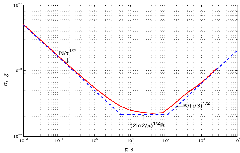
Fig. 8. Allan variance of accelerometer noise
