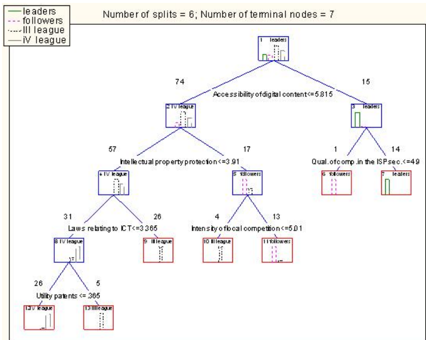
Fig. 2. Decision tree for the Environment factor
