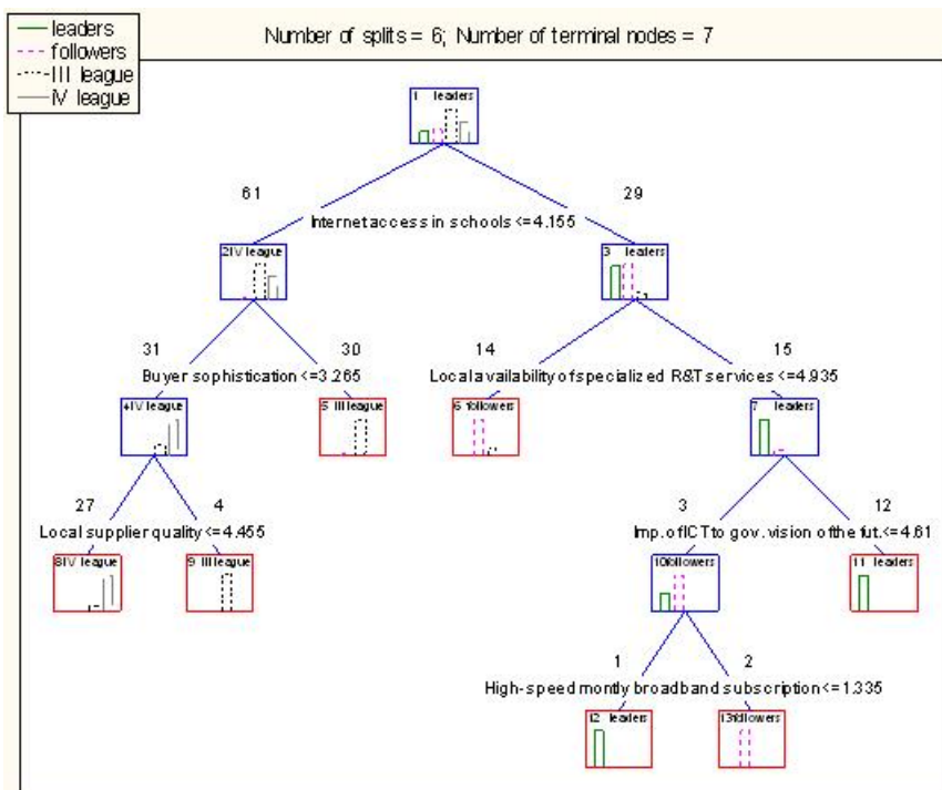
Fig. 3. Decision tree for Readiness factor
