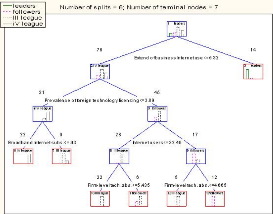
Fig. 4. Decision tree for Usage factor
